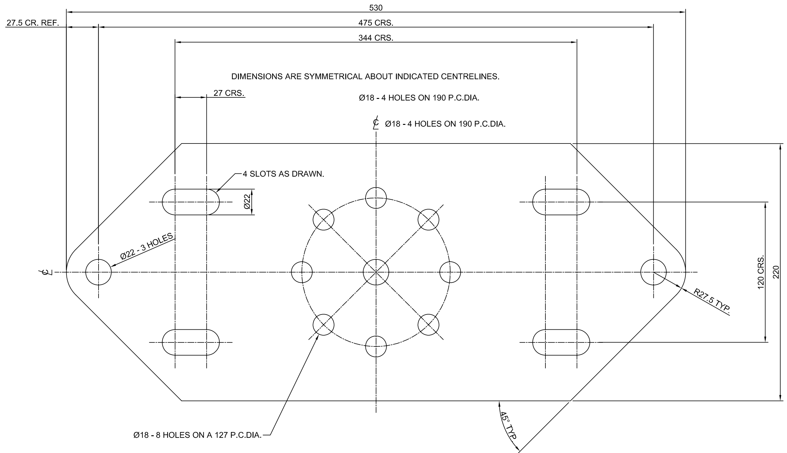
ITEM 1. 530 LONG x 220 WIDE x 15 THICK FLAT BAR.
